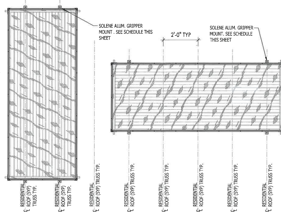
TYPICAL COLLECTOR ORIENTATIONS
