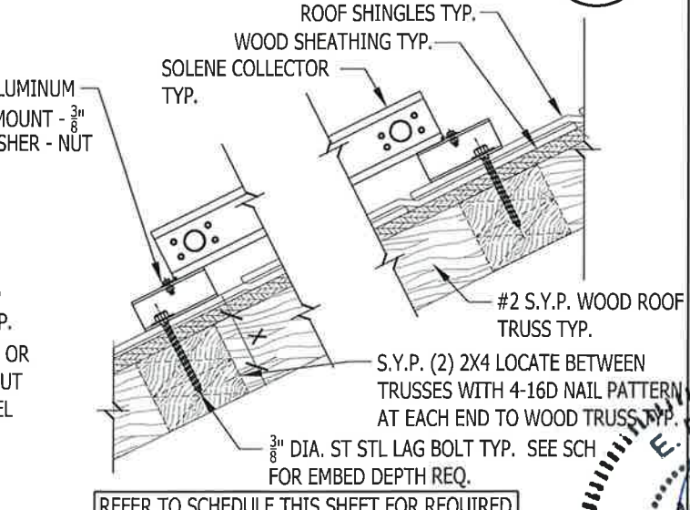
TYPICAL WOOD SPANNER OPTION FOR UNALIGNED TRUSS - GRIPPER MOUNT CONNECTION DETAIL
