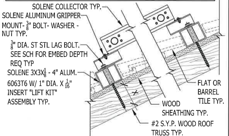
TYPICAL FLAT TILE - BARREL TILE ROOF CONNECTION DETAIL
