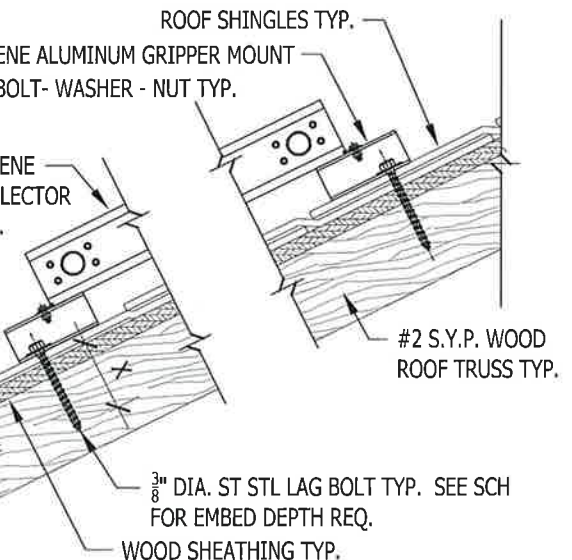
TYPICAL ASPHALT/METAL SHINGLE CONNECTION DETAIL
