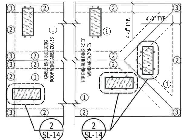
TYPICAL COLLECTOR PITCHED ROOF LAYOUT - WIND ZONES - SCHEDULE - PLAN
