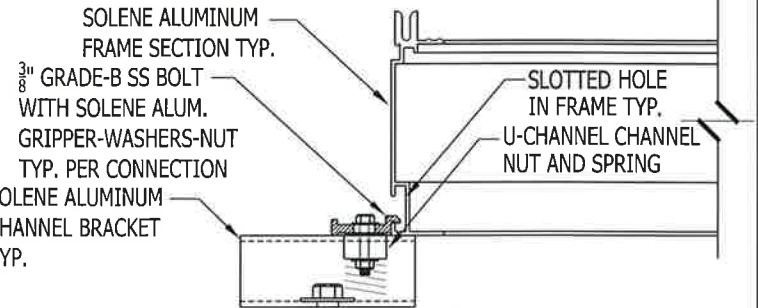
TYPICAL GRIPPER BOLT - FLUSH MOUNT DETAIL
