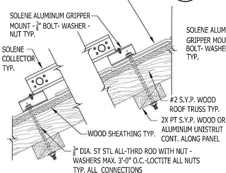
TYPICAL LIMITED SPACE OPTION CONNECTION DETAIL
