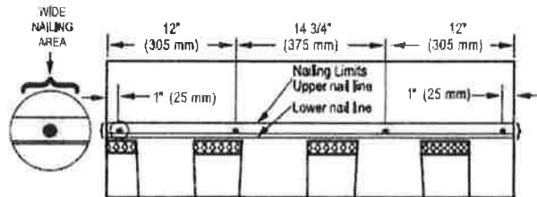
Nailing area for low and standard slopes (from 2:12 to 21:12) Nail between upper & lower lines as shown above.
