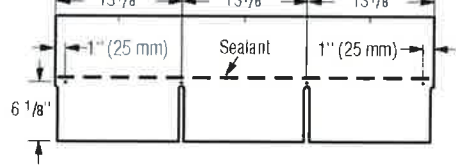
Figure 11-3: Use four nails for every full shingle.
