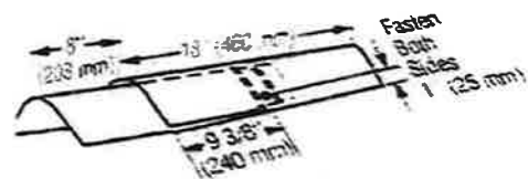
Figure 15-21: Installation of caps along hips and ridges.
