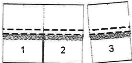
Figure 15-14: 12 three-piece units separate to make 5-1/4 Hatteras Accessory shingles.
