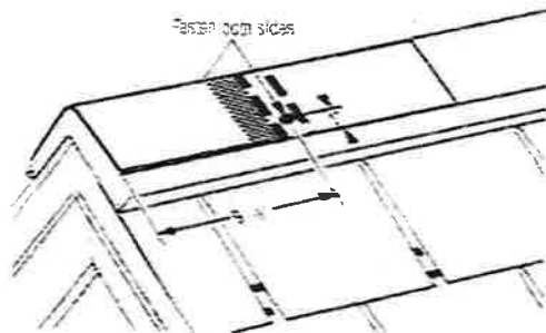
Figure 15-14: 12 three-piece units separate to make 5-1/4 Hatteras Accessory shingles.
