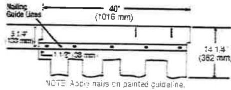
Figure 15-5: Fastening Presidential and Presidential TL Shake shingles on low and standard slopes.
