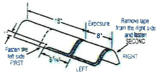
Figure 1-19: Installation of Shangle® Ridge shingles on hips and ridges
