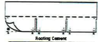
Figure 11-6: Use four nails and six spots of asphalt cement on steep slopes
