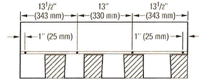
Figure 13-4: Use four nails for every full shingle.
