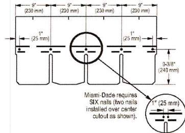
Figure 11-3: Use FIVE nails for every Highland Slate shingle.
