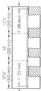
Figure 13-4: Use four units for every full shingle
